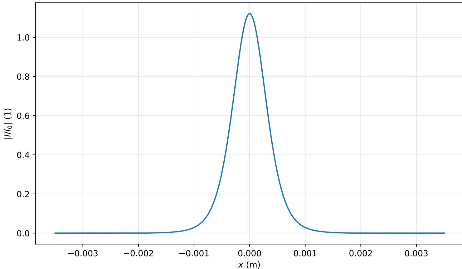
Intensity profile I(x, y = 0, z = 1.911m)/I_0 , P_{in}=0.7P_{cr} , artificial time
